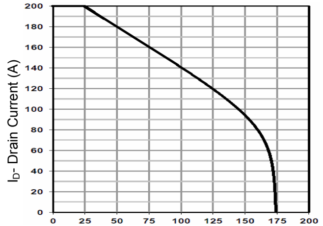
Figure 10 Current De-rating
